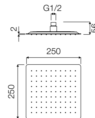
HKSO101C Soffione quadro Square showerhead 25x25 cm
