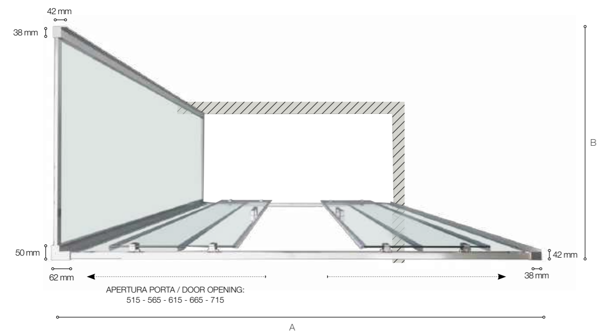
PORTA ABBINATA A LATO FISSO DOOR MATCHED WITH FIXED PANEL
