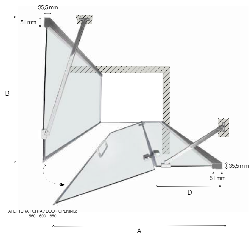
PORTA ABBINATA A LATO FISSO DOOR MATCHED WITH FIXED PANEL
