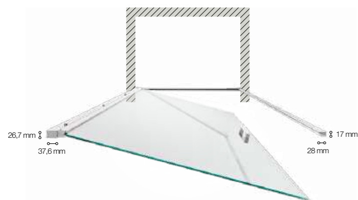
DIMENSIONI PORTA (A) (NICCHIA) CON PROFILO CHIUSURA NTPC03 DOOR SIZES (A) (NICHE) WITH CLOSING PROFILE NTPC03
