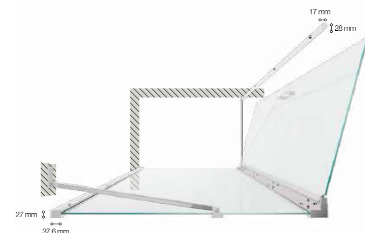
PORTA ABBINATA A LATO FISSO SALFIS DOOR MATCHED WITH FIXED PANEL SALFIS
