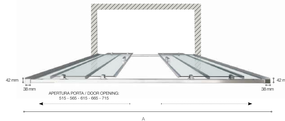
DIMENSIONI PORTA (A) (NICCHIA) DOOR SIZES (A) (NICHE)
