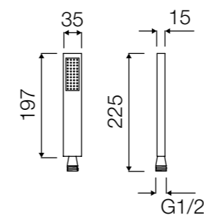
HKDOC130C Doccetta quadra Square handheld showerhead
