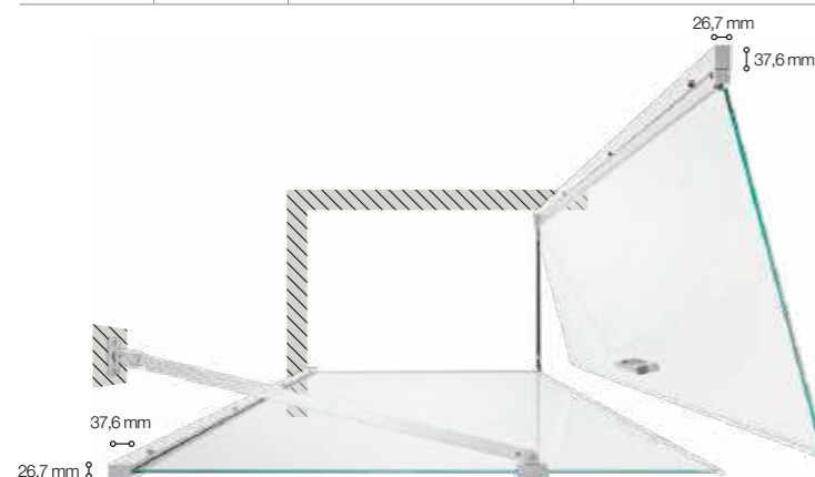
PORTA ABBINATA A LATO FISSO PARETE DOOR MATCHED WITH FIXED PANEL PARETE
